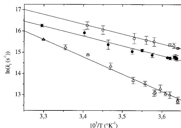
FIGURE 8 Arrhenius plots for the protonation reactions of carboxylates at pH 7.0 (○) and 4.5 (●) and of histidines at pH 7.0 (Δ). Results of the interpolation with straight lines are reported in Table 2.
