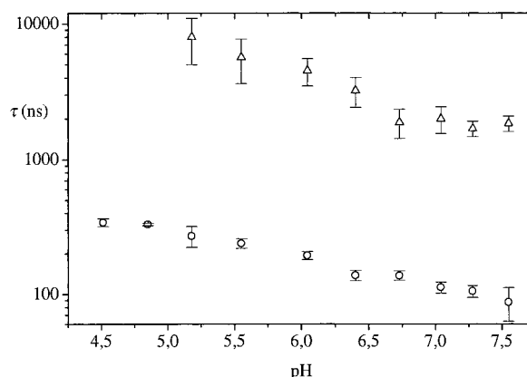
FIGURE 4 Prepulse pH dependence of lifetimes of the structural volume changes of an aqueous solution of oNBA and ApoMb determined by deconvolution of volumetric signals acquired at T = 1.79^\circ\text{C} . Absorbance of the solution (due only to oNBA) at 355 nm was 0.4 (1 cm path length), [\text{ApoMb}] = 80 \mu\text{M} , [\text{GuHCl}] = 0.2 \text{ M} . Plots report \tau_2 ( \circ ) and \tau_3 ( \triangle ).
