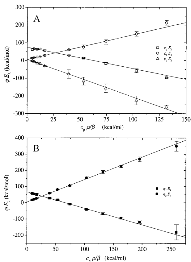
FIGURE 7 Energy content of the transient species ( \phi_i E_\lambda ) as a function of the thermoelastic parameter C_p \rho / \beta of the solution. (A) pH 7.0, [ApoMb] = 50 \mu M, [GuHCl] = 0.2 M; (B) pH 4.5, [ApoMb] = 58 \mu M [GuHCl] = 0.2 M. For both samples, the absorbance of the solution (due only to oNBA) at 355 nm was 0.4 (1 cm path length). Symbols are explained in the figure. The results of the linear interpolation for each transient are reported in Table 2.
