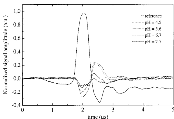
FIGURE 2 Volumetric signals of an aqueous solution of oNBA and ApoMb at T = 1.79^\circ\text{C} at different prepulse pH values. Absorbance of the solution (due only to oNBA) at 355 nm was 0.4 (1 cm path length), [\text{ApoMb}] = 80 \mu\text{M} , [\text{GuHCl}] = 0.2 \text{ M} . The reference compound (BP) signal was acquired at 5.0^\circ\text{C} .
